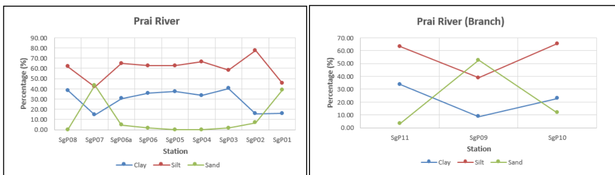
Figure 3: Particle size distribution in sediments at Perai River and its subsidiary
