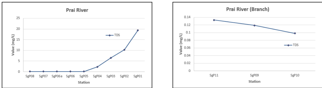
Figure 2: Physical parameters at Perai River and its subsidiary
