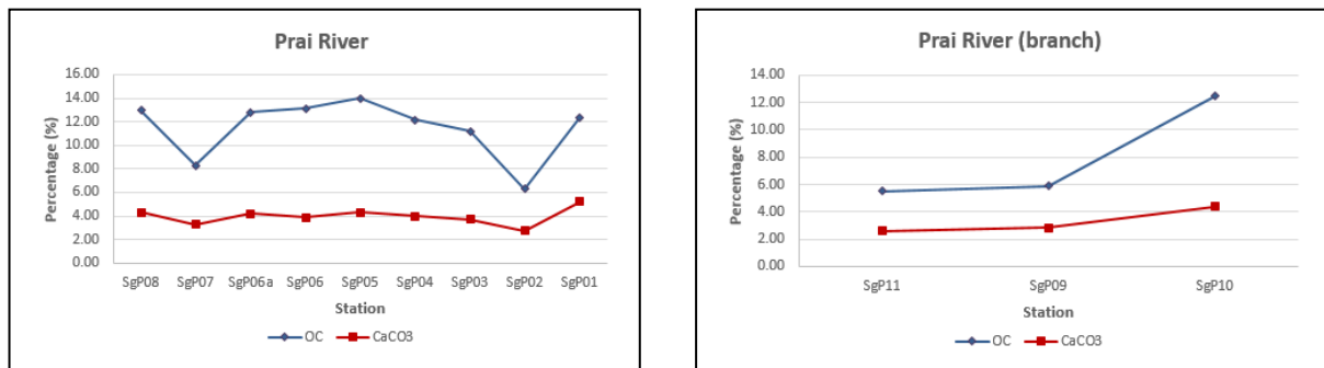
Figure 4: Organic carbon and carbonate distribution in sediments at Perai River and its subsidiary
