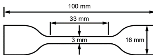
Figure 2: Dimension of dumbbell cut sample
